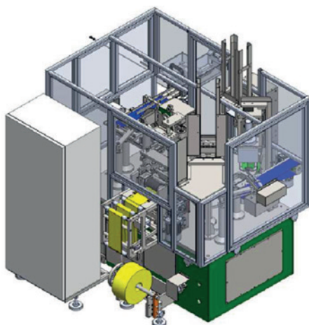
BTR 10 - Packaging machine. Bundling butter for tray and hood. Product: butter size hotel
