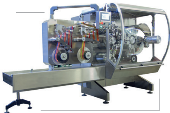
Wrapping machine for stock tablet and cubes at speed 1000 Continuous motion Change size from the tablet to the cube and vice versa
